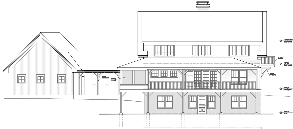
EXTERIOR ELEVATIONS
