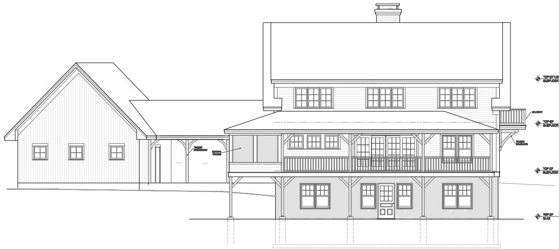
EXTERIOR ELEVATIONS
