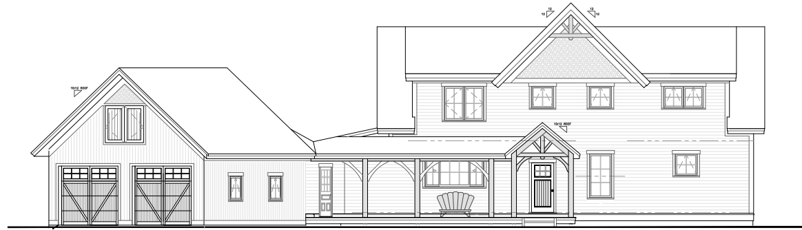
EXTERIOR ELEVATIONS
